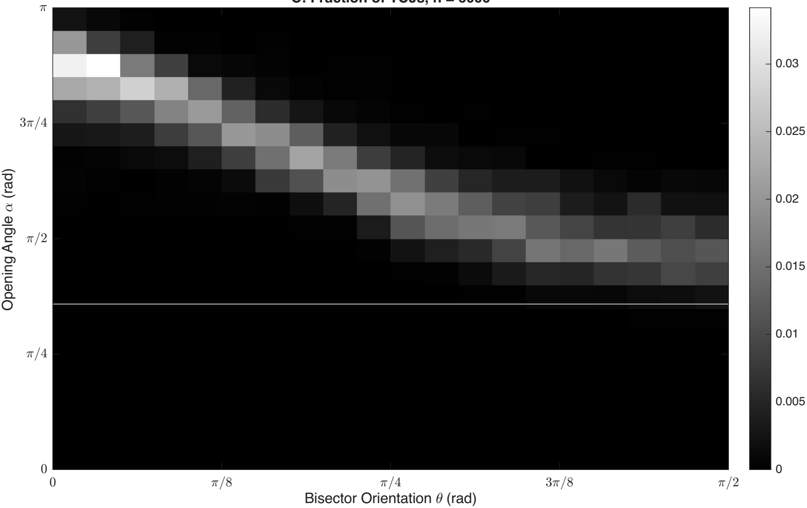
C: Fraction of TCJs, n = 6000
